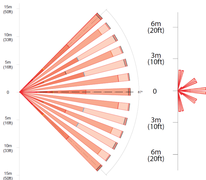
Figur 1: Toppvy
